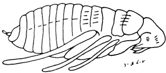
Fig. 101. Pupa of dog flea, Ctenocephalides canis (Curtis).
